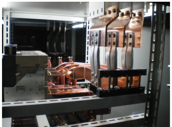
Main Circuit in narrow space
