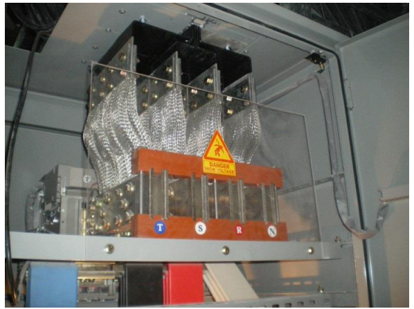
Bus Way lead to Terminal
