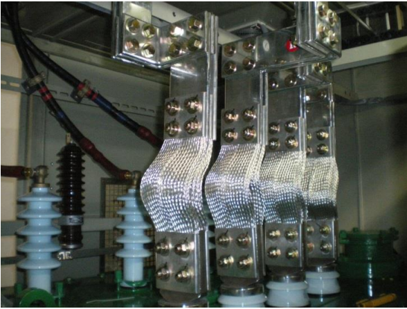
Transformer lead to Terminal
